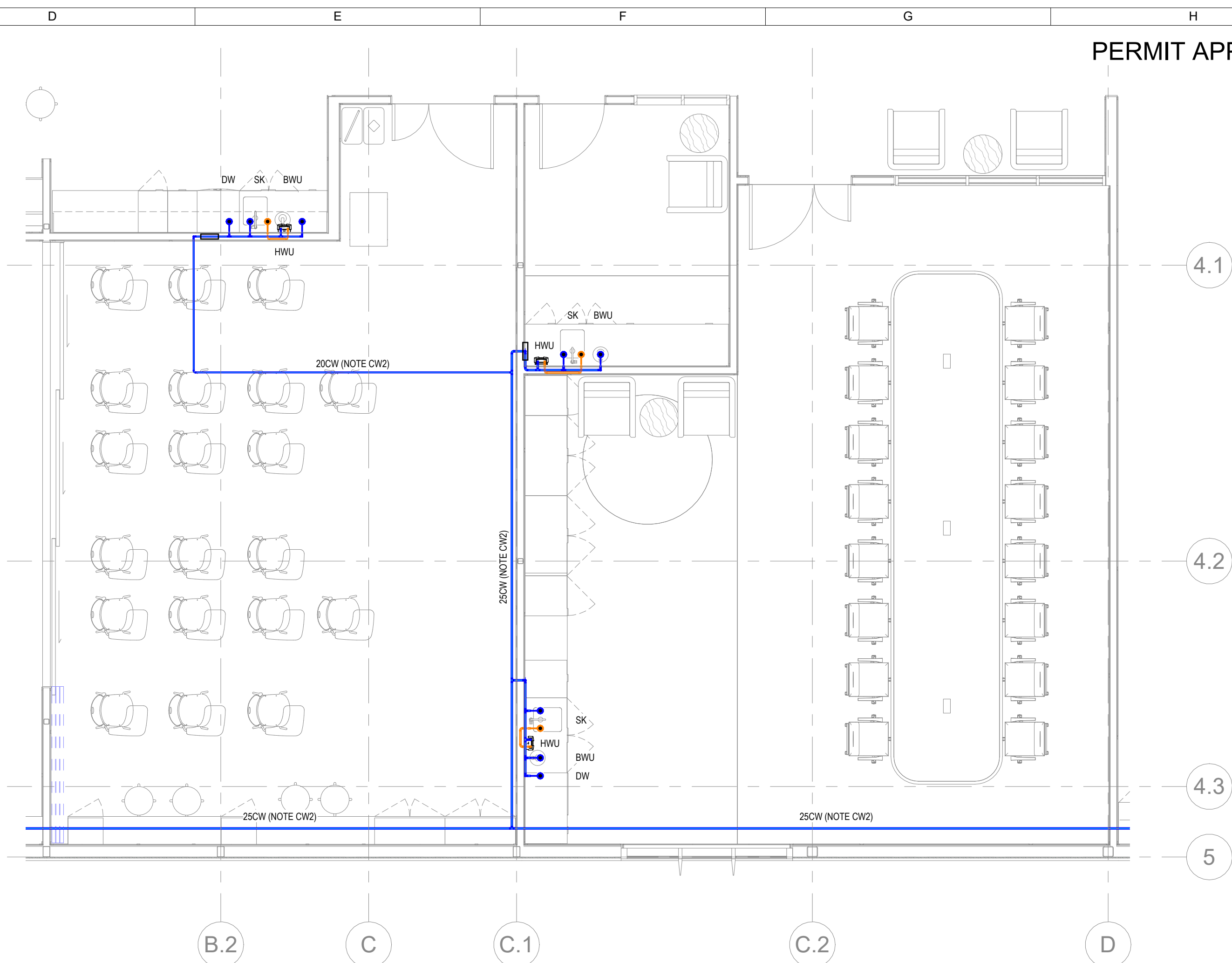
GROUND FLOOR TRAINING KITCHEN WATER LAYOUT - INSET 03
